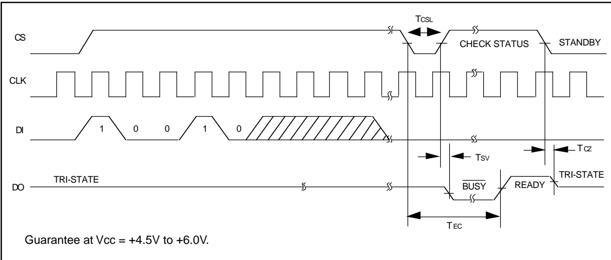
FIGURE 2-8: ERAL TIMING
