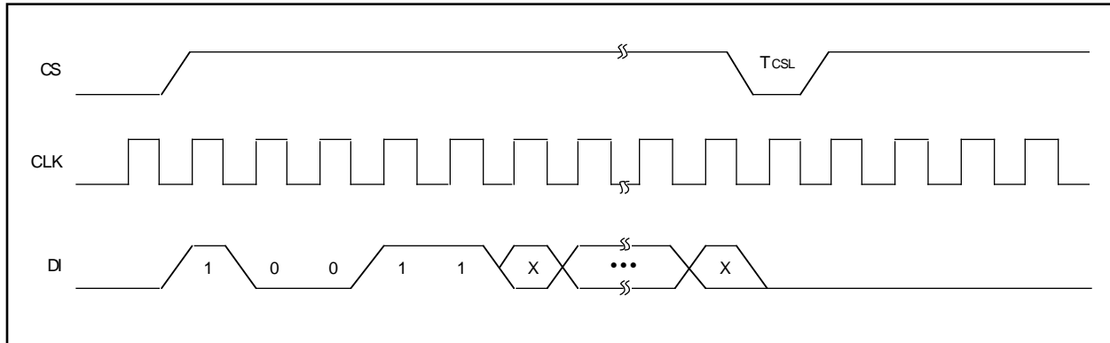
FIGURE 2-4: EWDS TIMING
