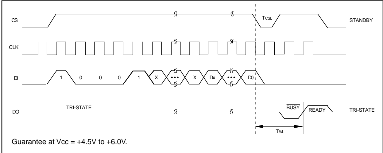
FIGURE 2-7: ERASE TIMING
