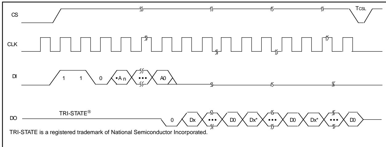
FIGURE 2-2: READ TIMING
