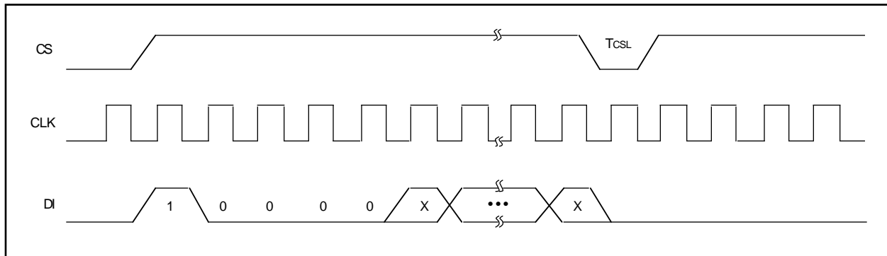
FIGURE 2-5: WRITE TIMING
