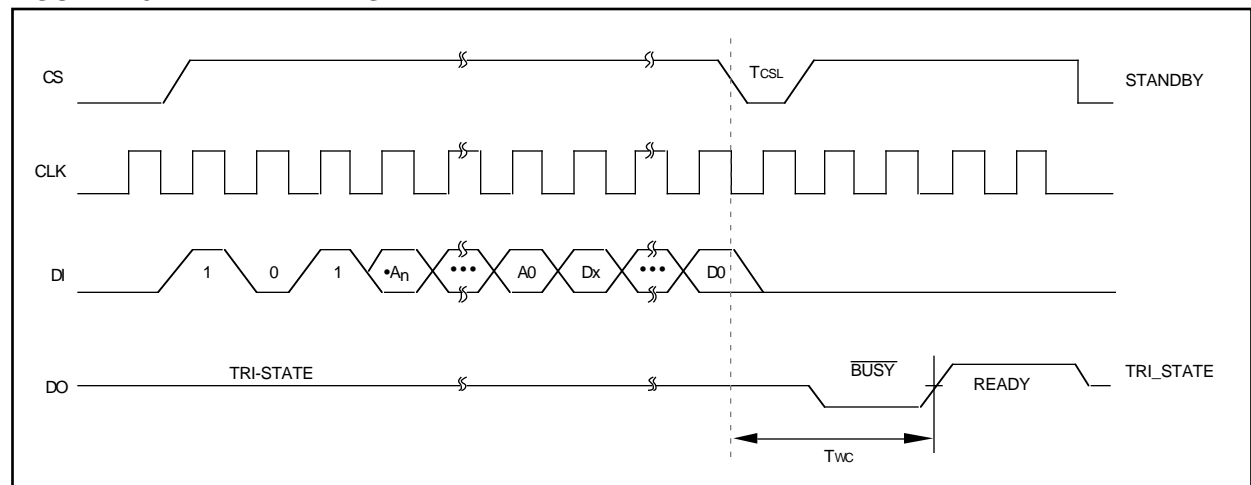
FIGURE 2-5: WRITE TIMING
