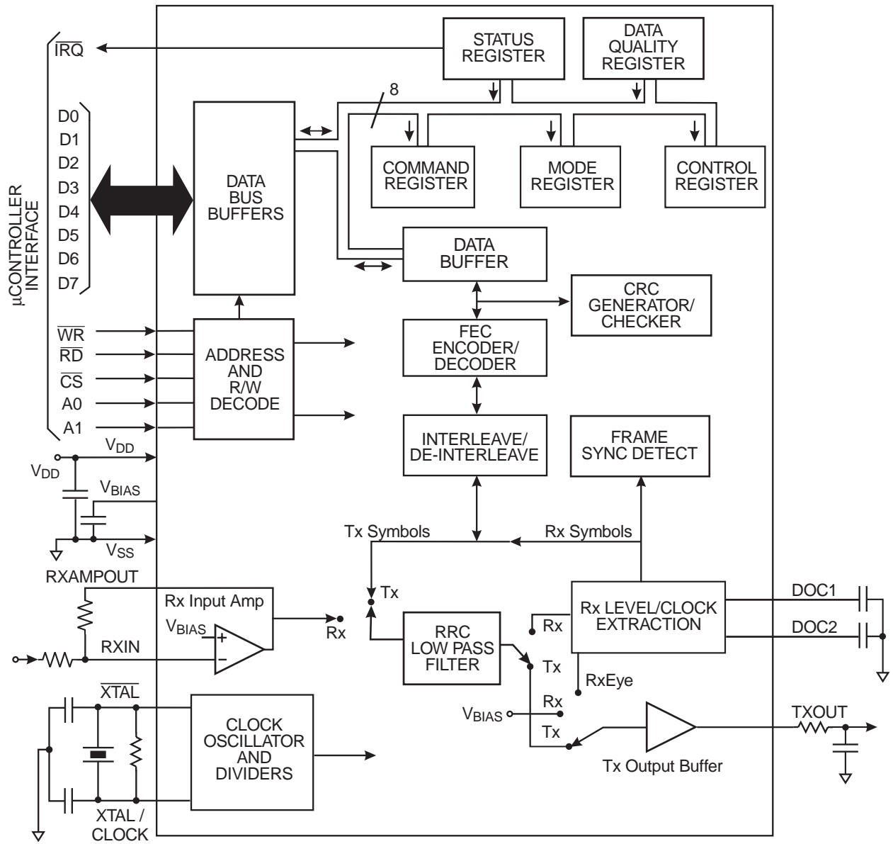
Figure 1: Block Diagram
