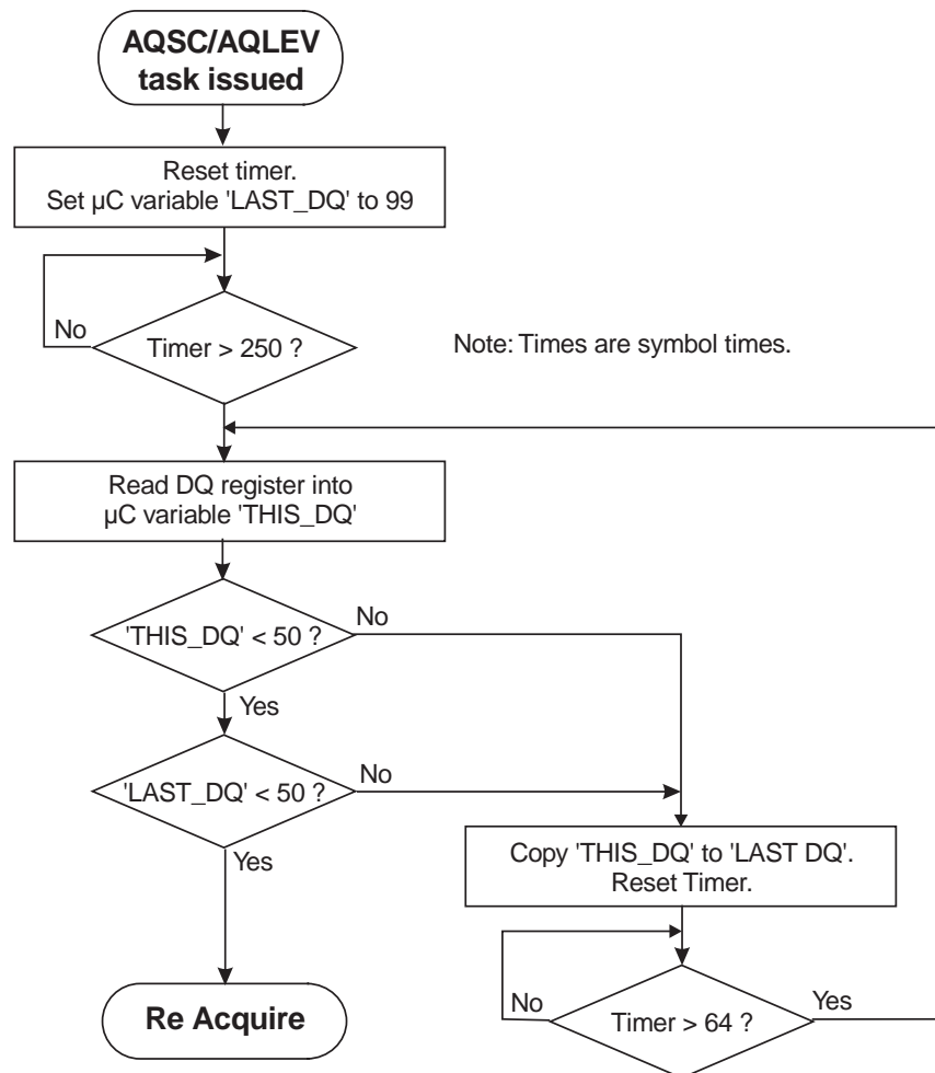
Figure 27: Received Signal Quality Monitor Flowchart
